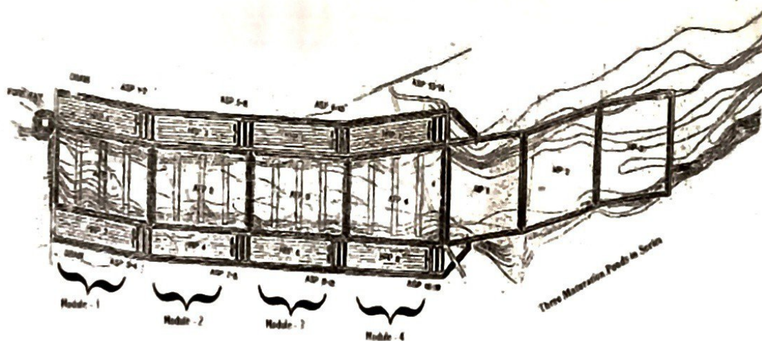
Figure 5. Schematic map of AIWPS facility proposed at Sota showing four modules in parallel and three maturation ponds in series. AFP, Advanced facultative pond; HRP, High rate pond; ASP, Algal settling pond and MP, Maturation pond.
